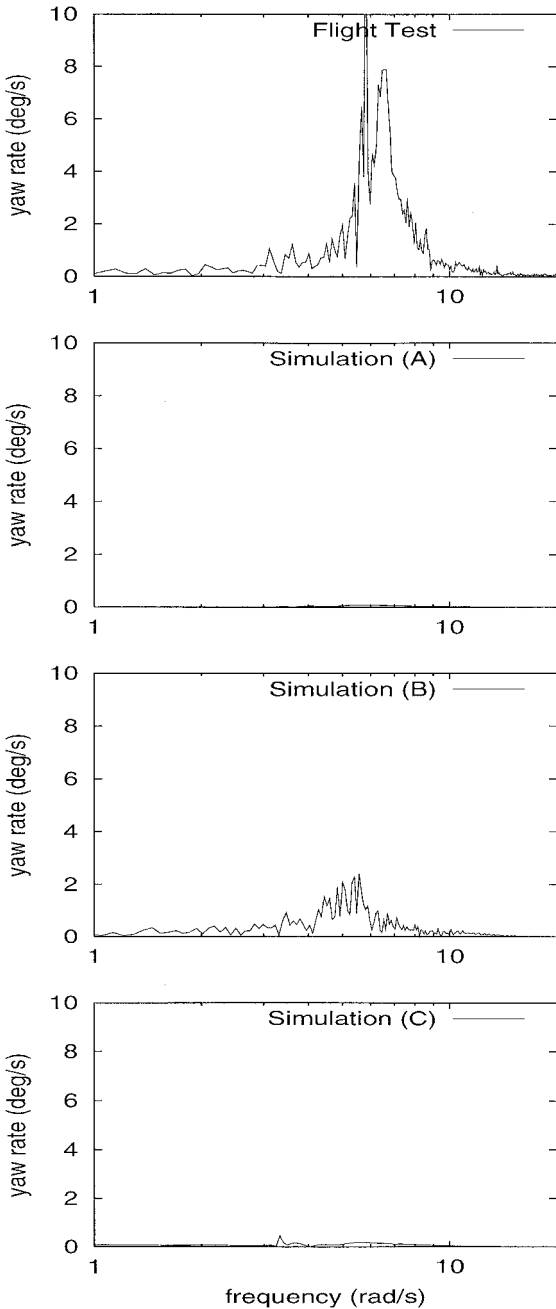
Fig. 6 Comparison of the yaw rate r frequency-domain results of simulation with flight-test data, drogue parachute deployment.
