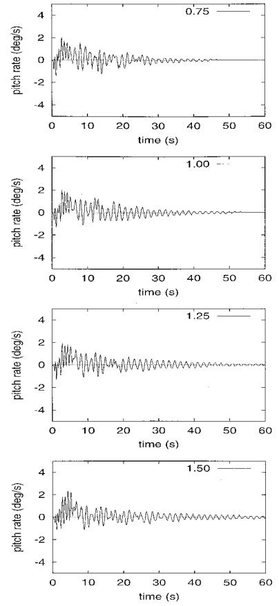
Fig. 13 Effect of riser length ratio l_r/l_{r0} on the pitch rate q_P of the parachute, main parachutes deployment, mode A.
