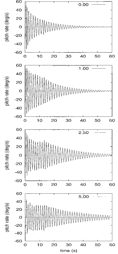
Fig. 14 Effect of parachute added mass ratio m_{ax}/m_{ax0} on the pitch rate q of the capsule, main parachutes deployment, mode A.
