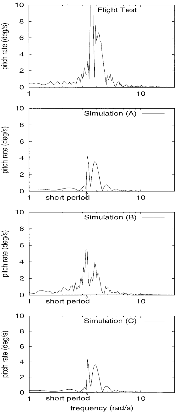
Fig. 5 Comparison of the pitch rate q frequency-domain results of simulation with flight-test data, drogue parachute deployment.
